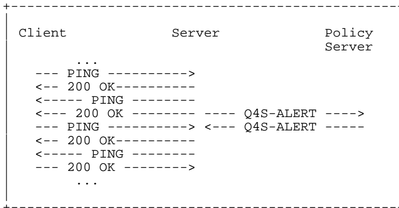
Figure 12 Continuity in policy-server alerting mode
