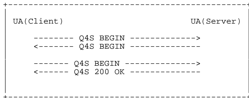
Figure 14 P2P roles.
