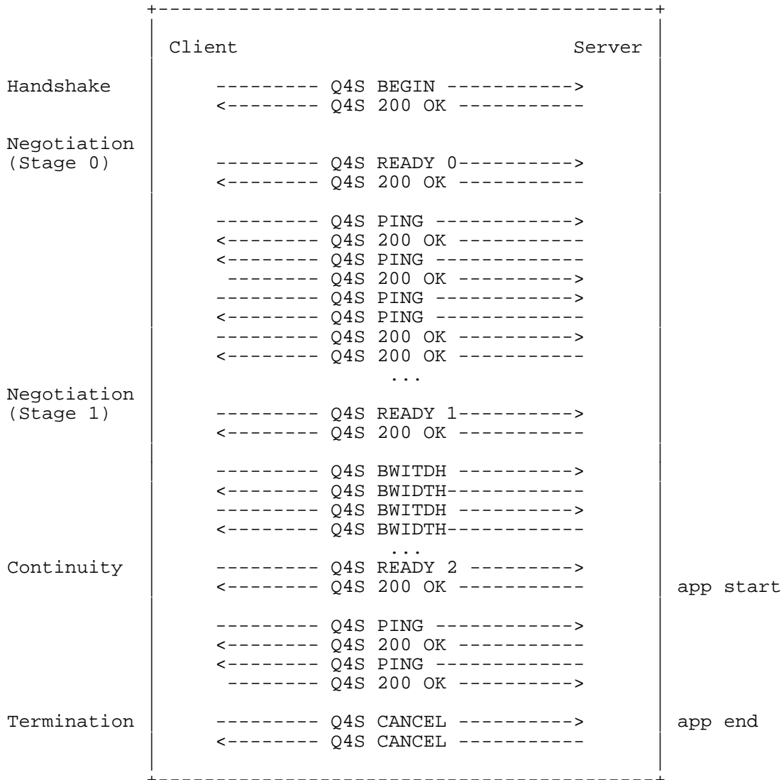
Figure 1 Successful Q4S message exchange.
