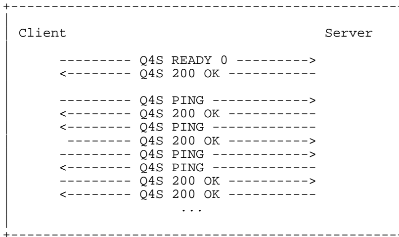
Figure 7 Simultaneous exchange of PING request and responses.
