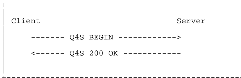
Figure 6 Handshake phase.
